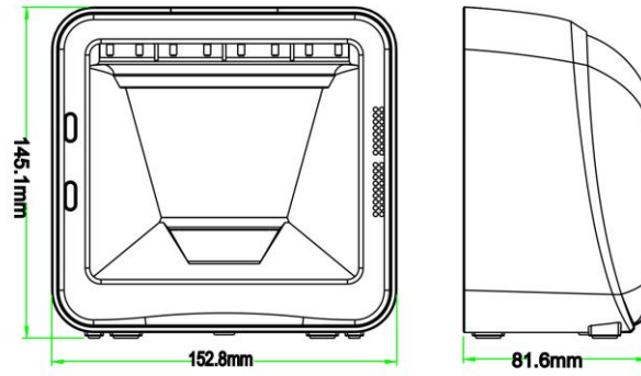
Figure 2-2 Dimensions (without stand)
