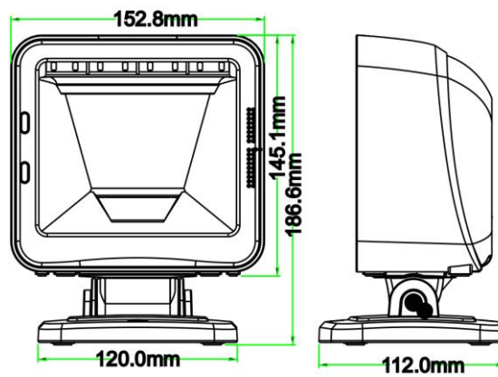
Figure 2-3 Dimensions (with stand)
