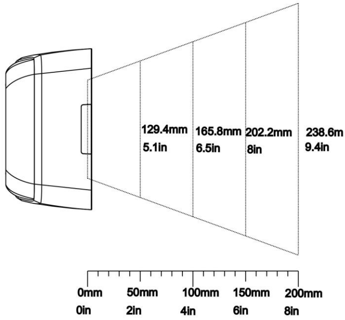
Figure 2-7 Field of view – Horizontal
