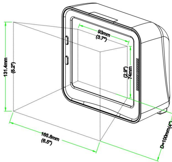
Figure 2-5 Field of view
