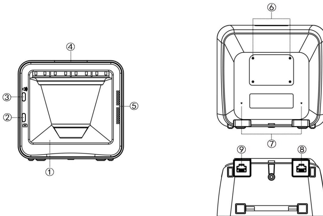
Figure 2-9 Parts of image platform
