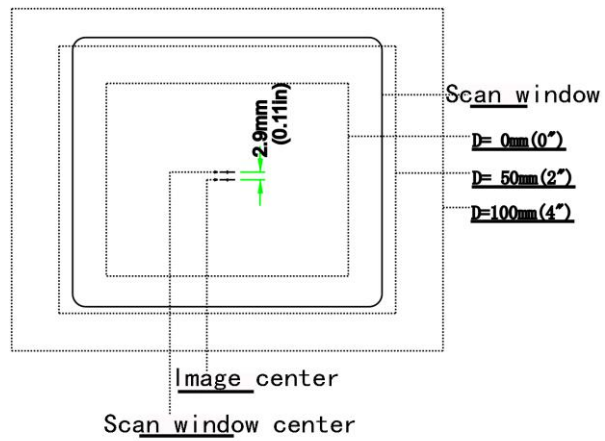
Figure 2-6 Field of view – Front view
