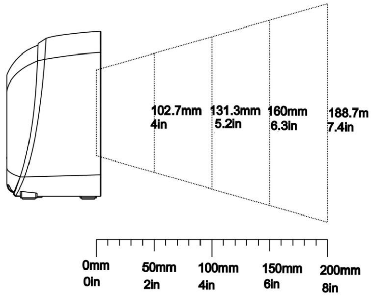
Figure 2-8 Field of view – Vertical
