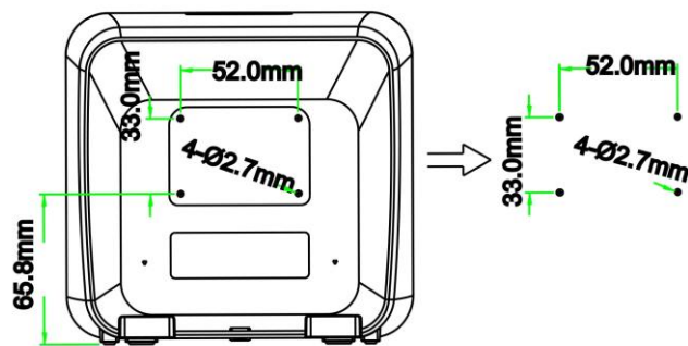
Figure 2-4 Dimensions of hanging holes
