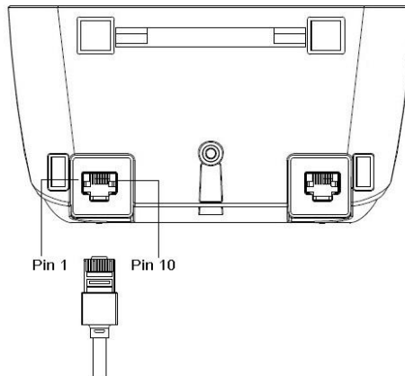
Figure 2-1 Cable connector interface pin-outs
